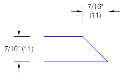
Section At Beveled Edge
